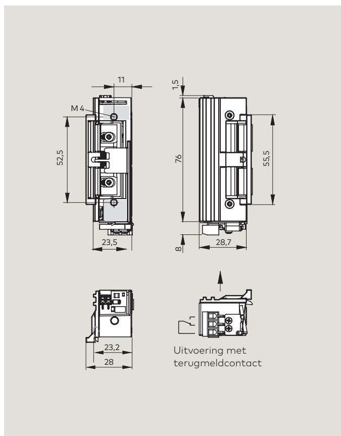
Fire 448 + Easy Adapt
