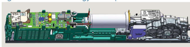
Fig. 1.2 ED50 low energy OHC operator
