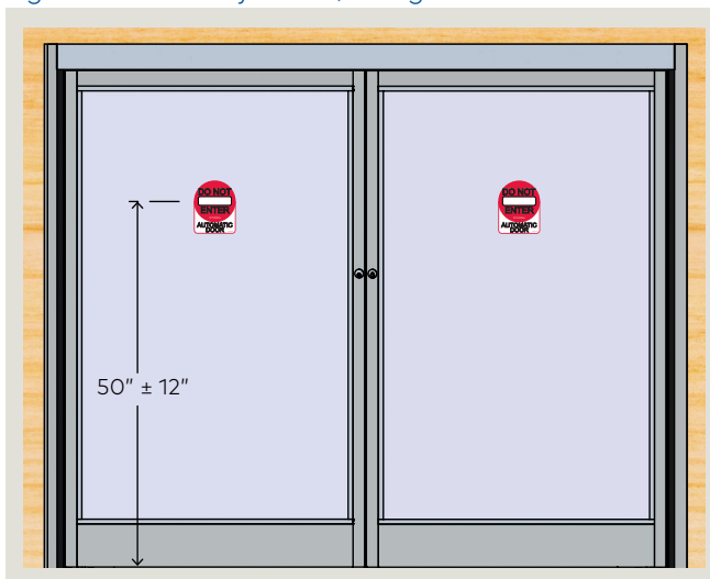
Fig. 7.5.4 One way traffic, swing side
