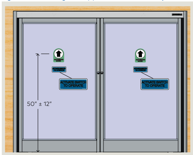
Fig. 7.5.3 Knowing act, approach side, one way
