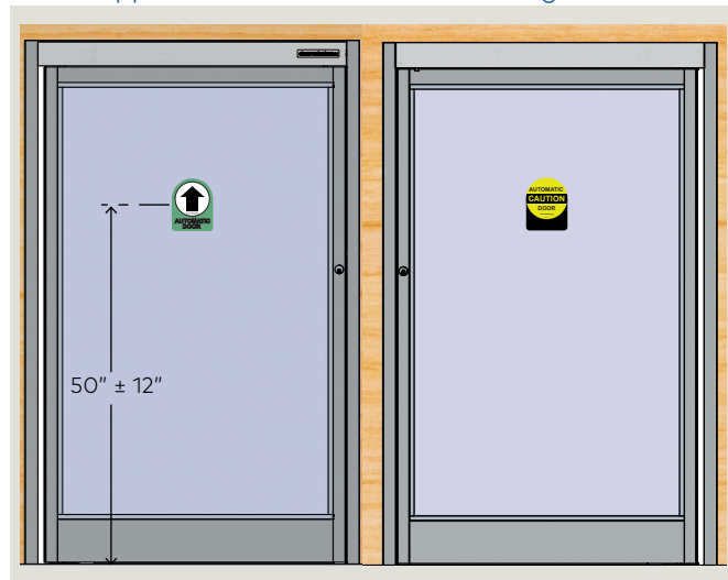
Fig. 7.3.4 Two way traffic
