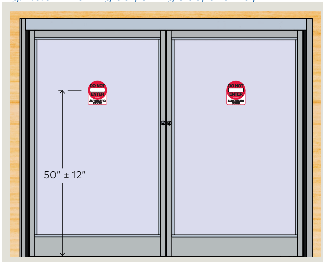
Fig. 7.5.6 Knowing act, swing side, one way
