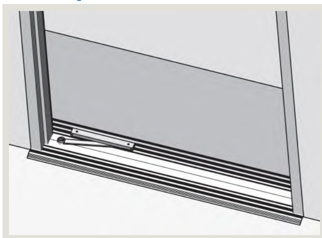
Fig. 8.1.2 Door threshold installation example for ED250 in-ground
