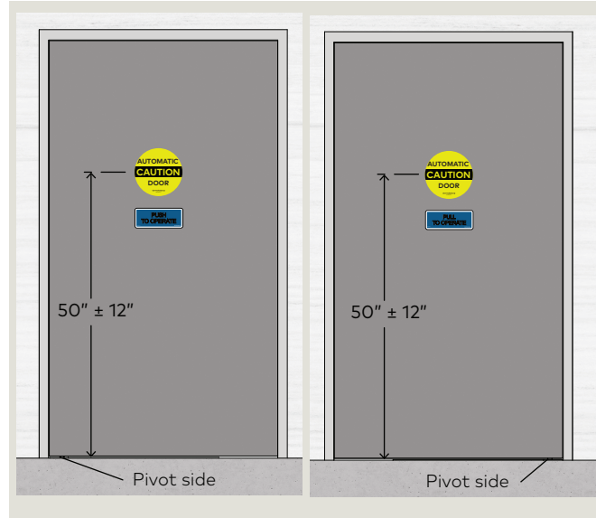
Fig. 7.3.2 Push/Pull Push To Operate
