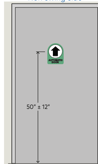
Fig. 7.4.2 Two way traffic Non swing side
