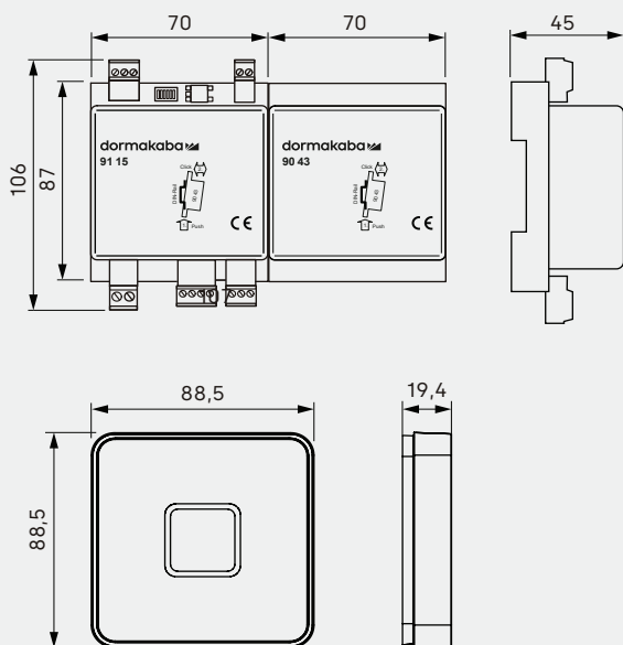
Wireless update reader: Remote reader 91 15 and an extension module 90 43 combined with a registration unit 90 01 as an example (dimensions in mm)
