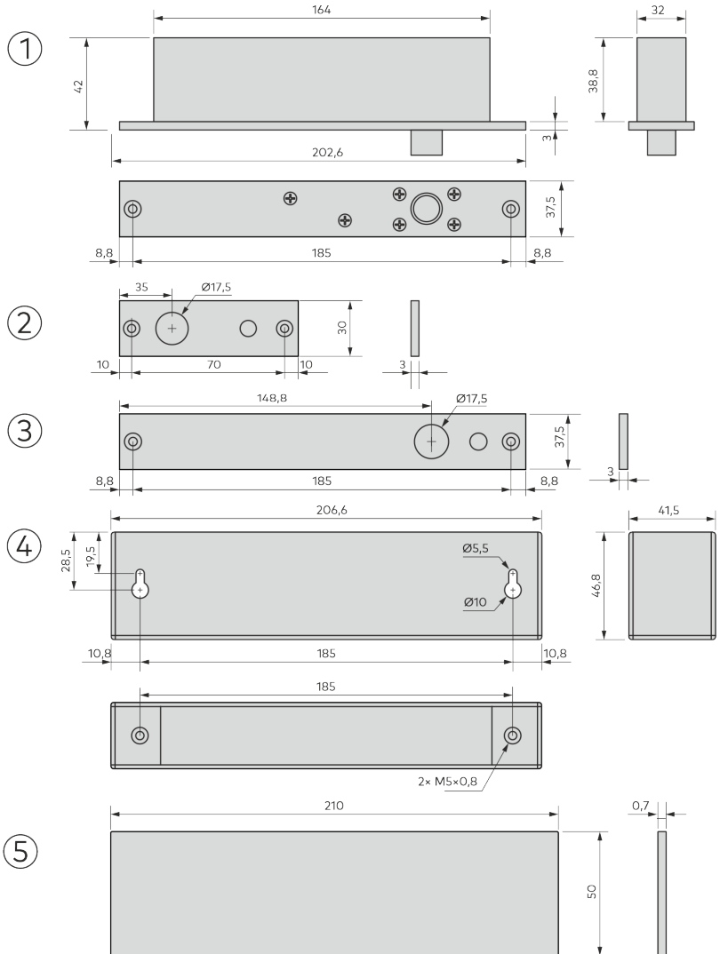
Fig. 2: Lock - dimensions
