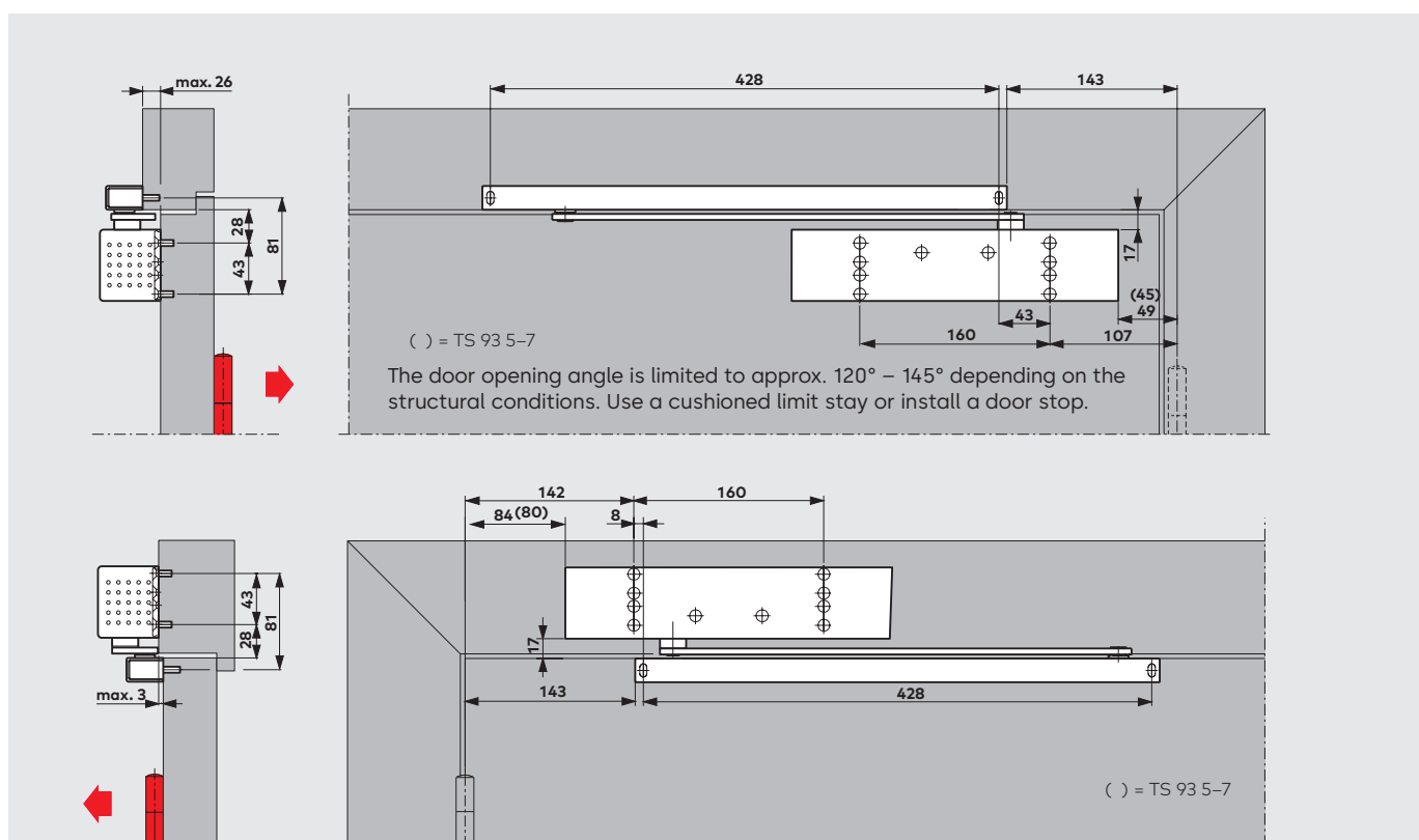
TS 93 G door closer with G-N slide channel assembly, door leaf fixing on the push side and transom fixing on the pull side. Examples: Anticlockwise-closing (ISO 6) door; mirrored arrangements apply to clockwise-closing (ISO 5) doors.
