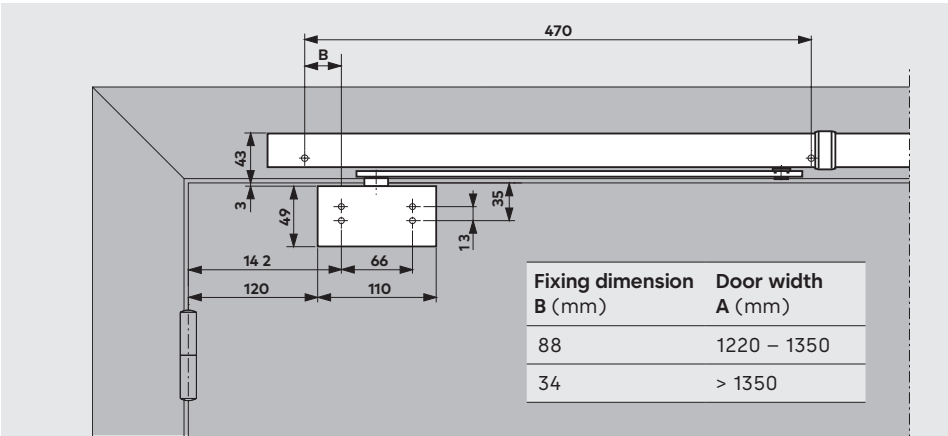
ED 100/ED 250 automatic swing door operator with G-SR door co-ordinator and G-SR pivot block
