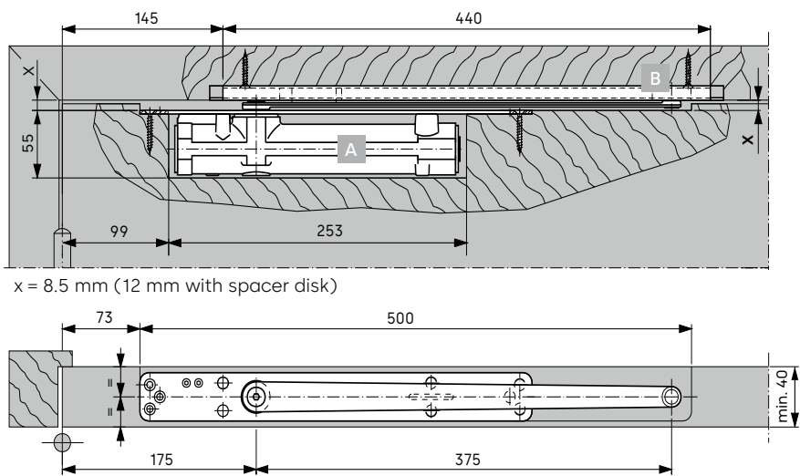
Installation example ITS Home with slide channel G 96 N20 in a solid-wood door
