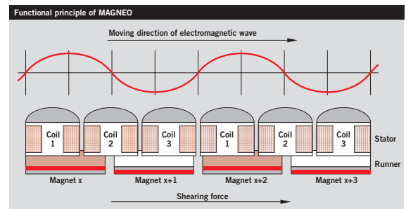
MAGNEO—driven by linear magnetic drive (LMD) technology
