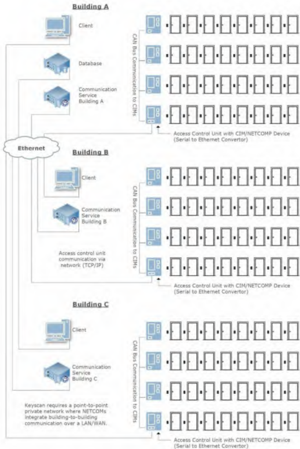
Figure 4 – Multiple Servers with a Third Building Added
