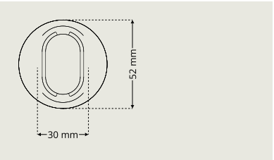
DAK 7340/D7320
