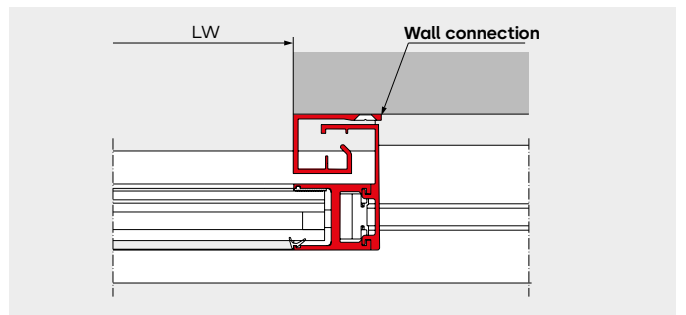
Wall connection
