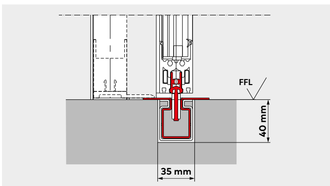
Floor guide
