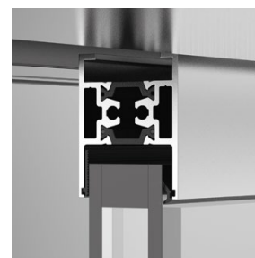
SST Flex Green Slim profile system with improved thermal separation
