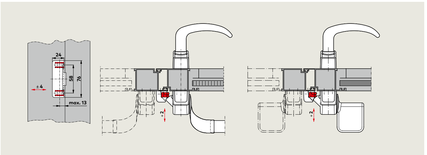
Application example of a PHX 21 on a door with flush meeting stiles, universal applicability for single-leaf and double-leaf
