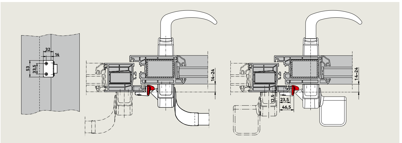
Application example of a PHX 22 on an over-rebated door, universal applicability for single-leaf and double-leaf doors
