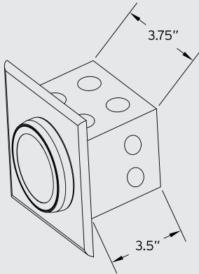
Screwless RCU flush mount
