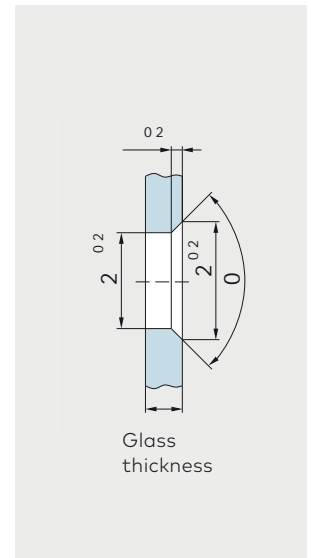
Countersunk bore for countersunk single-point fixings
