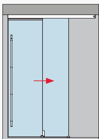
Glass door (8 - 13.5 mm) with glass overpanel and glass side lights (10 - 19 mm) - 2 and 4 panels
