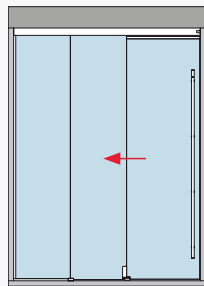
Glass door (8 - 13.5 mm) for the installation at ceiling / with side light (10 - 19 mm) - 2 and 4 panels
