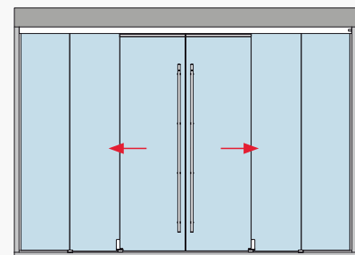
Glass door (8 - 13.5 mm) with glass overpanel and glass side lights (10 - 19 mm) - 2 and 4 panels
