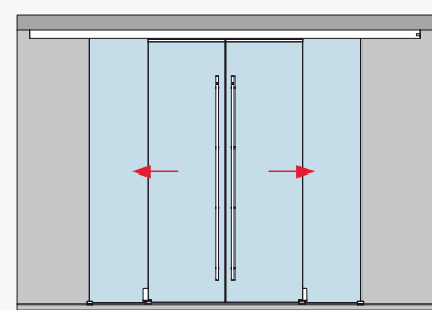
Glass door (8 - 13.5 mm) for the installation at ceiling / with side light (10 - 19 mm) - 2 and 4 panels
