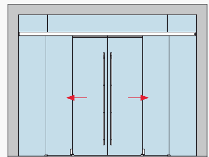
Glass door (8 - 13.5 mm) with glass overpanel and glass side lights (10 - 19 mm) - 2 and 4 panels
