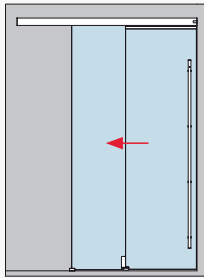
Glass door (8 - 13.5 mm) for the installation at ceiling / with side light (10 - 19 mm) - 2 and 4 panels
