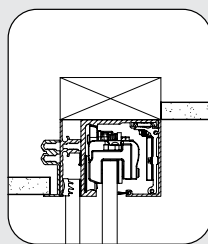
Option 7 Recessed, one side only
