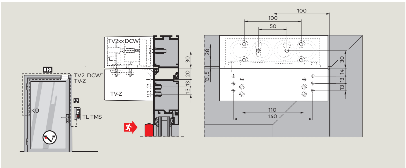
Installation on flush-closing door with TV-Z shim set on the door without limitation of the clear passage height, inward opening
