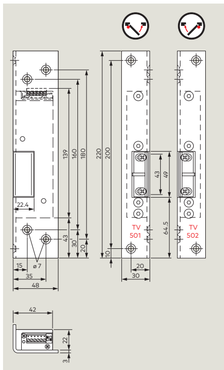
TV 501 DCW® / TV 502 DCW®
