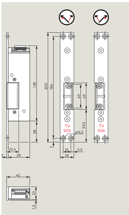
TV 505 DCW® / TV 506 DCW®
