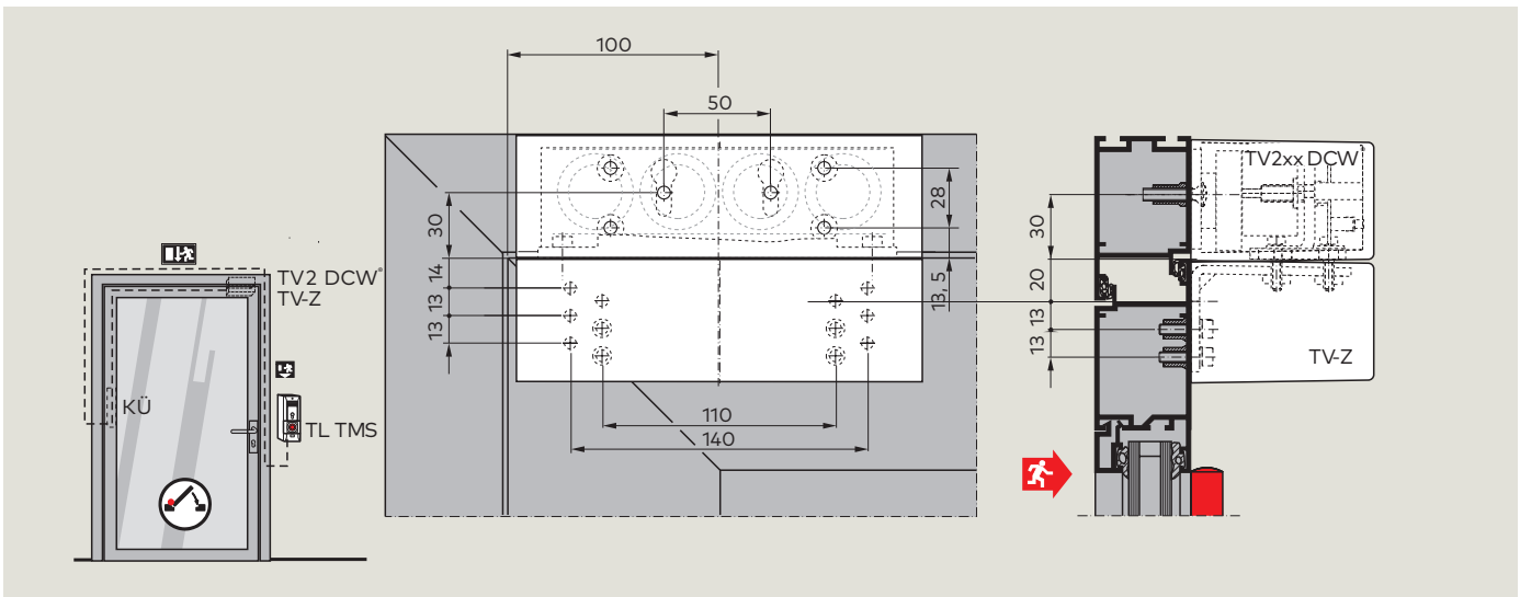
Installation on flush-closing door with TV-Z shim set on the door exterior, without limitation of the clear passage height, outward opening
