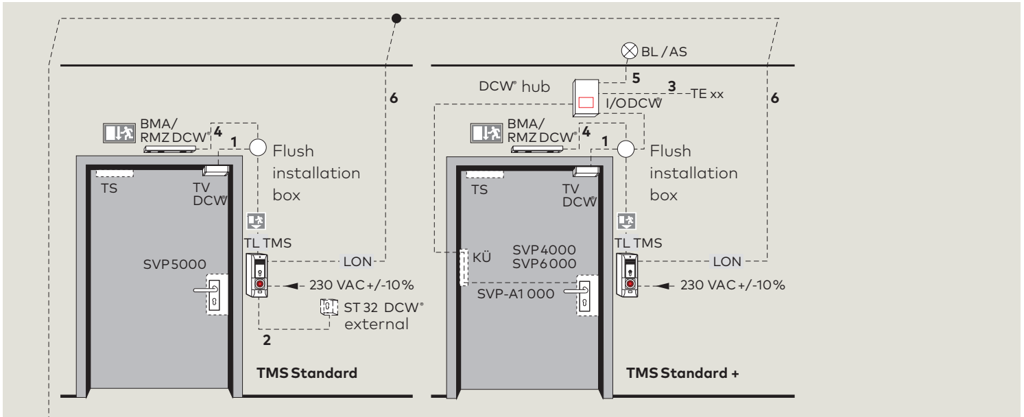
TMS Standard, anti-tamper monitoring contact, parameters freely configurable via PC
