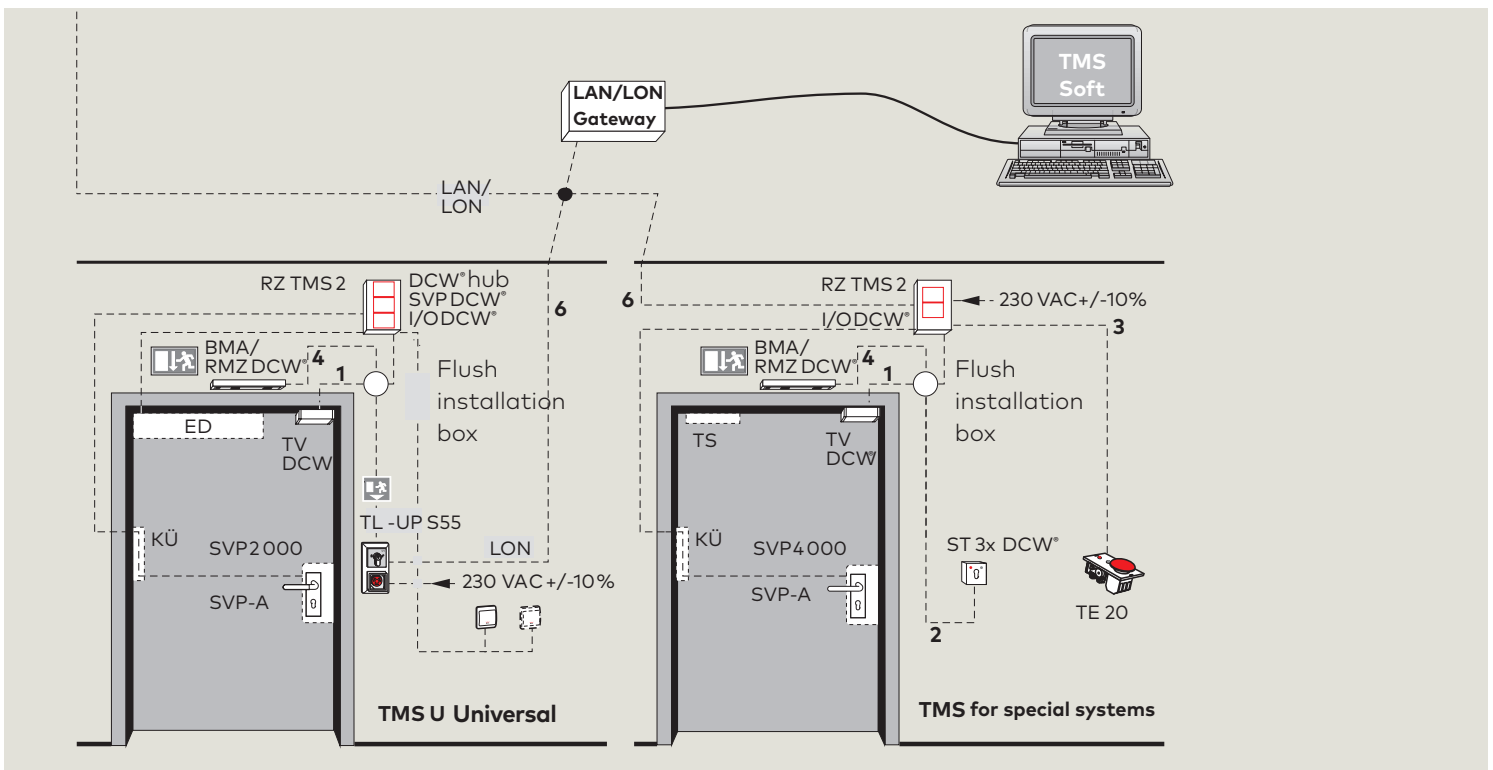
TMS Universal Design, anti-tamper monitoring contact, unlocking via lock cylinder of the SVP or access control reader, parameters freely configurable via PC
