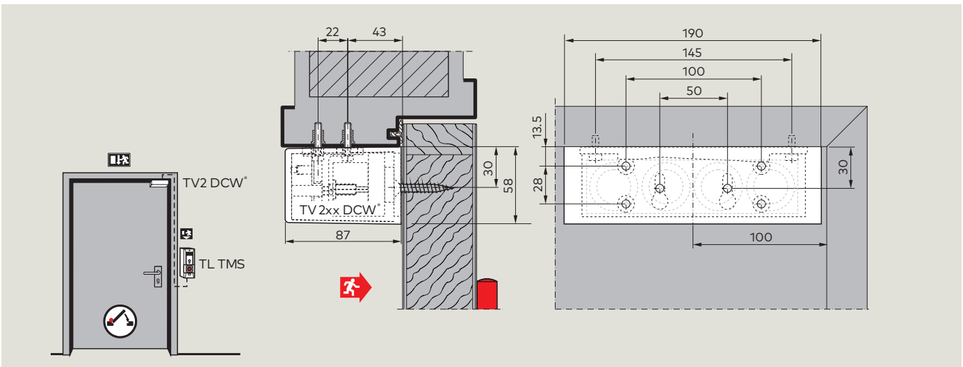
Installation in the frame reveal, outward opening
