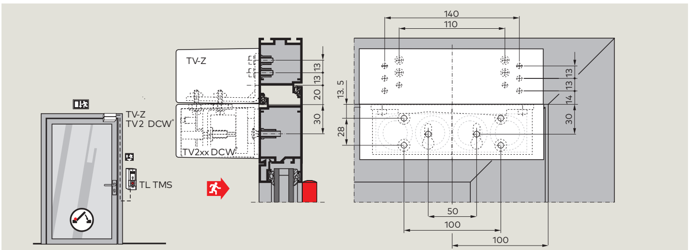
Installation on flush-closing door with TV-Z shim set on the frame, outward opening
