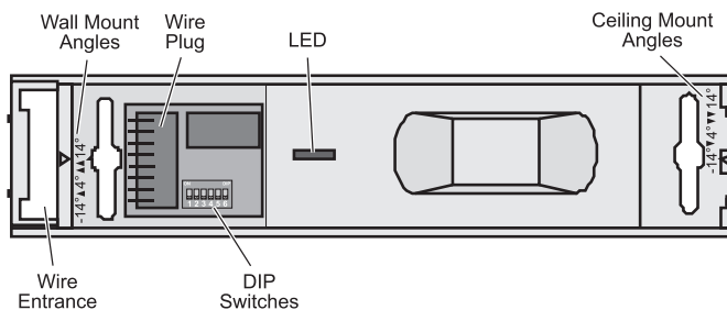
Fig. 1 Passive Infrared Egress Switch (front view)
