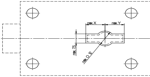
Fig. 3: Max. cross sectional area of keyhole
