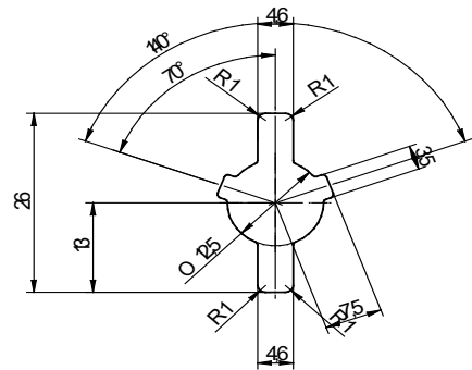
Fig. 2: Key carrier guide 86102
